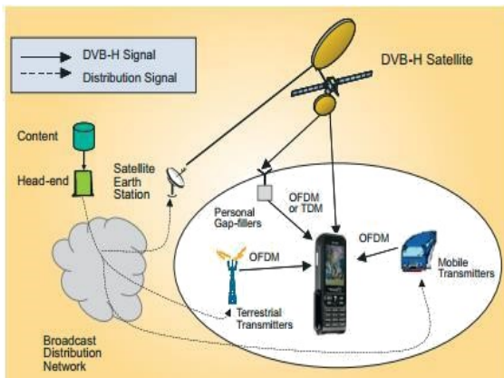
Fig 1. DVB-SH Architecture
