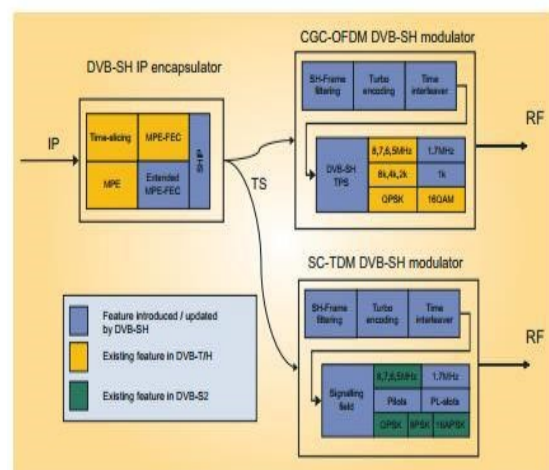
Fig 3. DVB-SH physical layer outline
