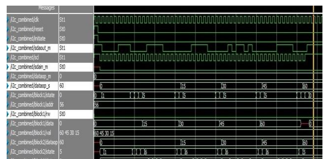
Fig 8. Simulation Result for Write operation 64 bits
