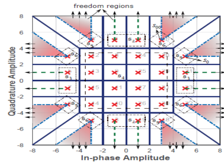
Fig 5. QAM Constellations
