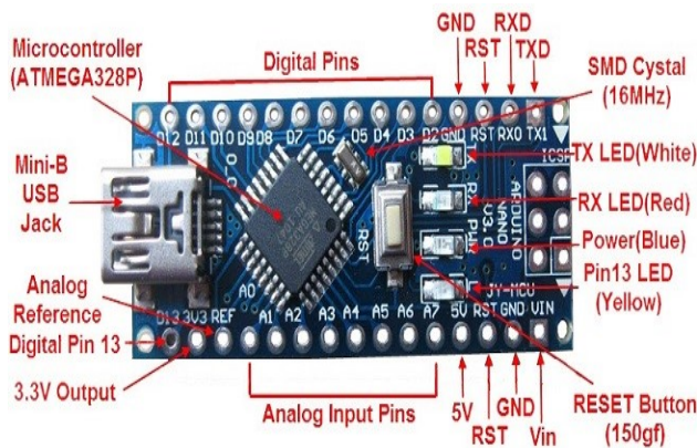
Fig 1. Pin diagram of Arduino Nano
