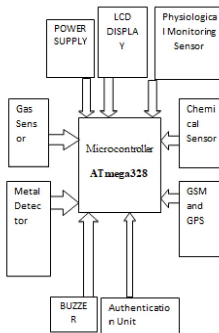
Fig 1. Block Diagram of Smart Army Jacket
